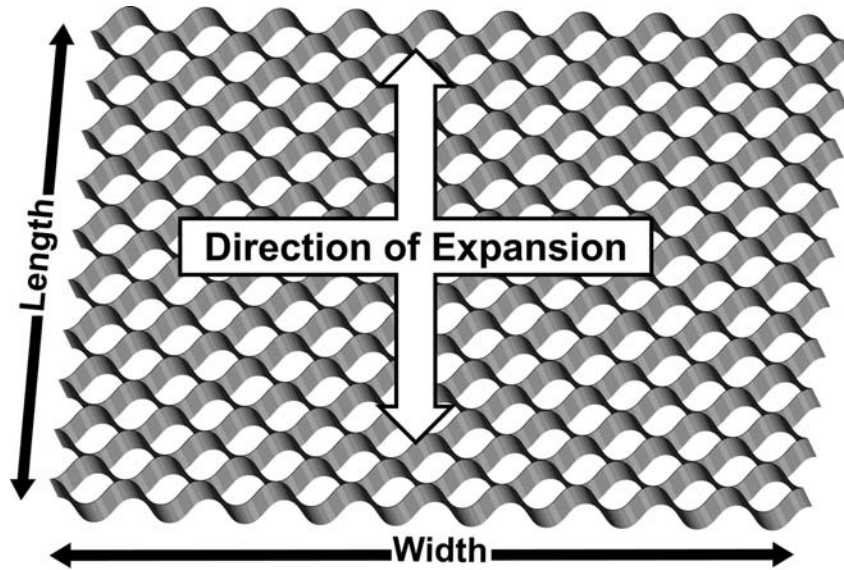
Figure 1 GC30V SSP GEOCELL Section
